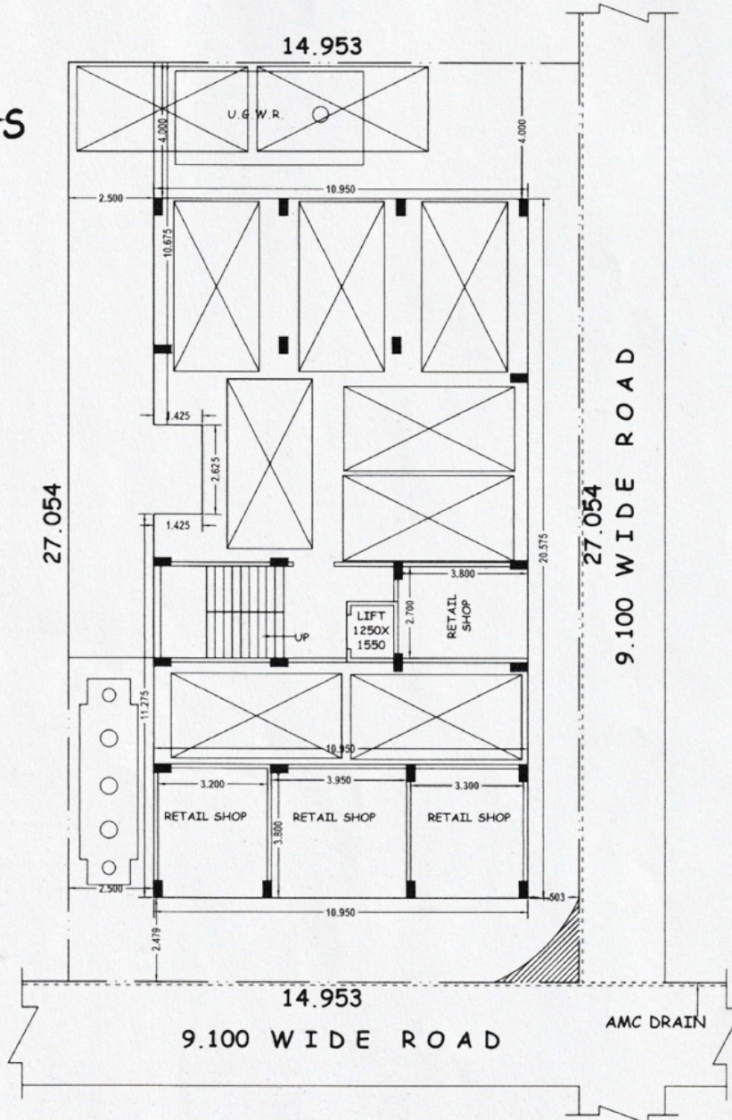
PROPOSED GROUND FLOOR SITE PLAN
